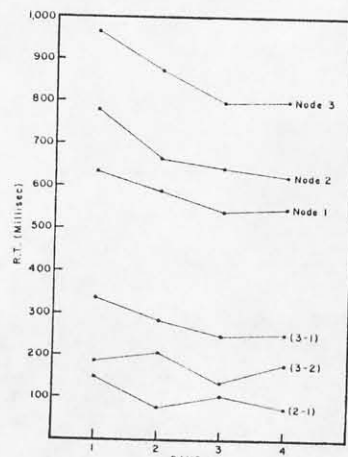
FIG. 3. Practice data for Experiment IV. (Lower curves refer to differences between nodes. Differences between Nodes 3-1 and 3-2 obtained by same - different subtractive method, for Node 2-1 same - same method was used.)
